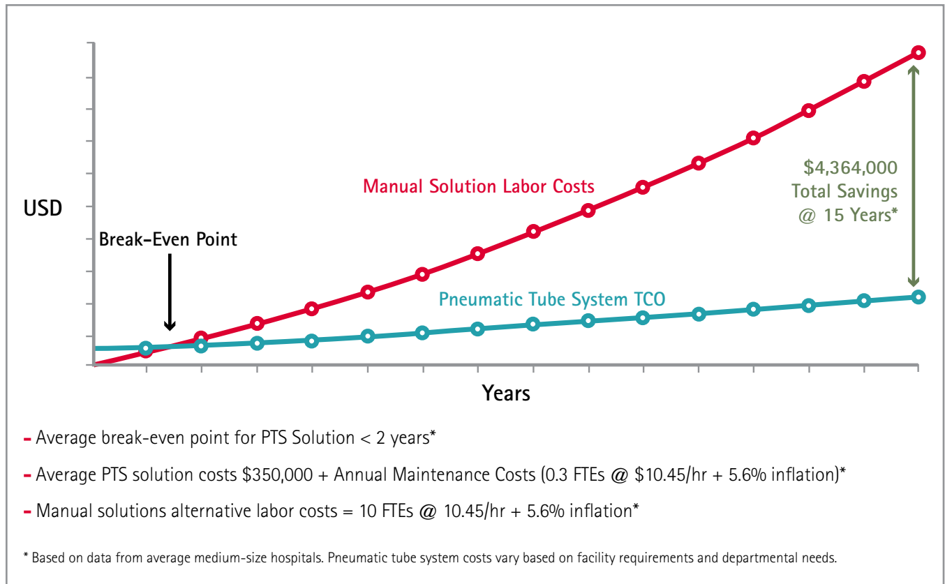
Figure 3: Comparing pneumatic tube system TCO to a manual solution over 15 years.
